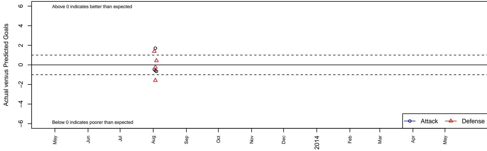
Explosion -Unk G01 Dots are actual minus expected GF (blue circles) and GA (red triangles). Blue line is smoothed change in attack strength. Red is smoothed change in defense strength.
